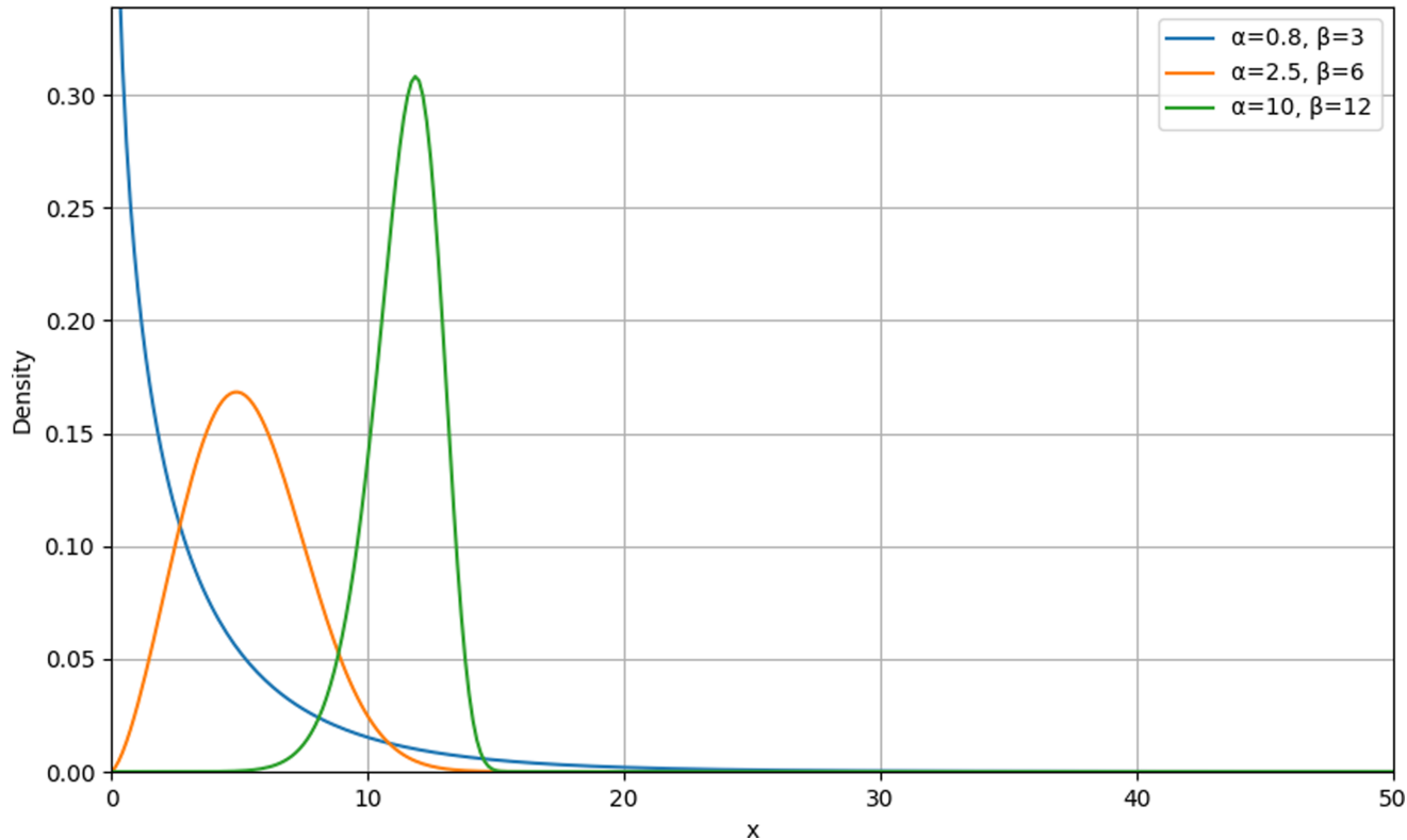
Figure 2 Weibull distribution density function curves under three different cases
