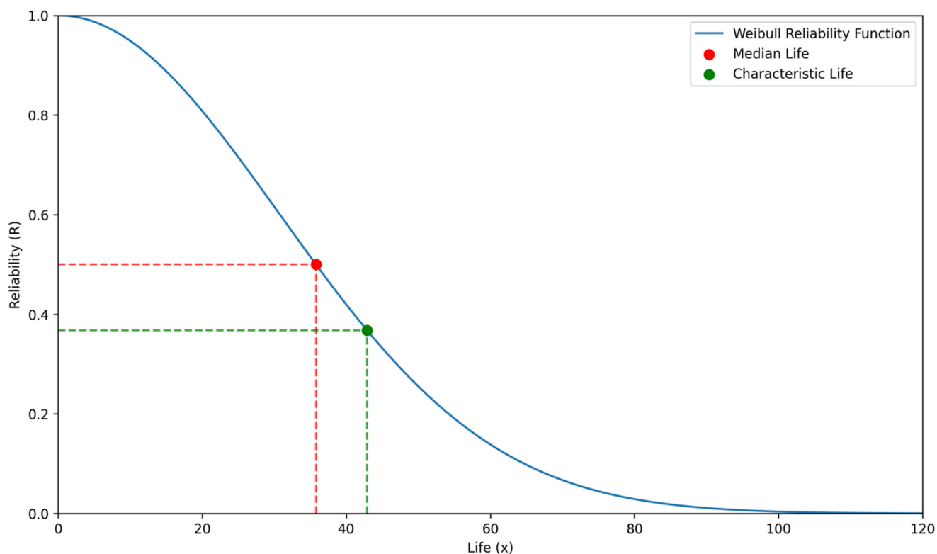
Figure 12 Characteristic life and median life corresponding to parameter estimates (2.0279 and 42.8871)
