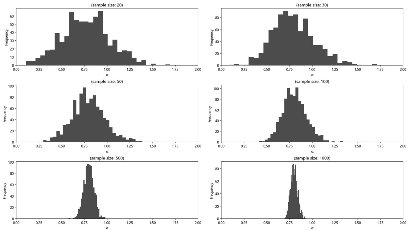
Figure 3 Frequency distribution histogram of \hat{\alpha} in case 1
