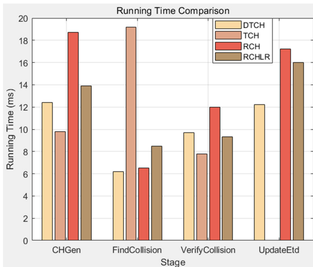
Figure 2 Computation cost of algorithms for DTCH
