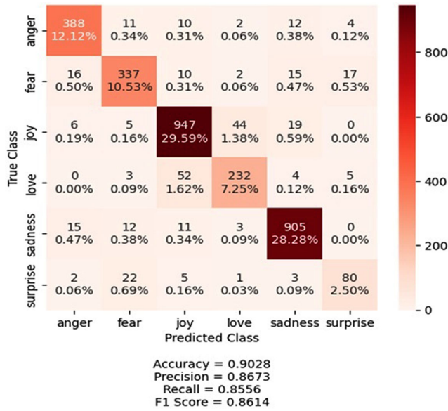
Figure 6 Confusion matrix for the proposed model
