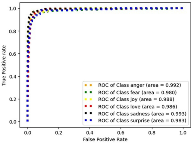
Figure 8 ROC curves of the proposed model
