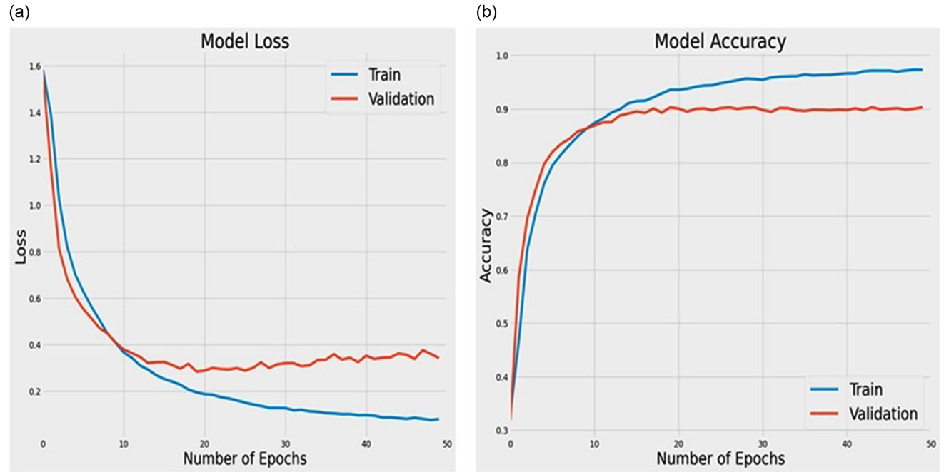
Figure 7 (a) Model loss curve and (b) model accuracy curve
