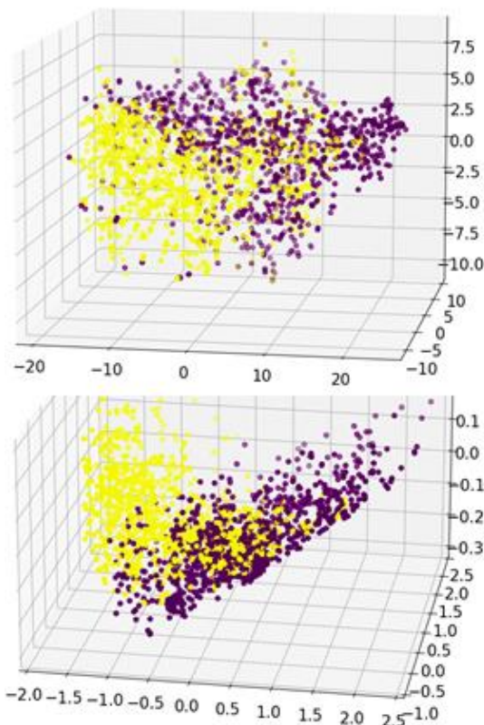
Figure 4 PCA transformation for primary features (top) and secondary features (bottom)
