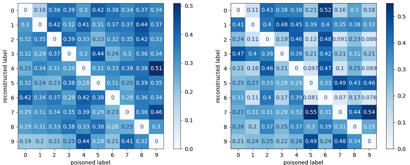
Figure 4 Average attack accuracy (AAA) for the combined reconstruction and poisoning attack (CRPA) across all combinations of generator and poisoning labels in the MNIST (left) and FMNIST (right) datasets. Each class in the datasets is assigned to a single participant, resulting in a total of ten participating clients over 300 global training rounds
