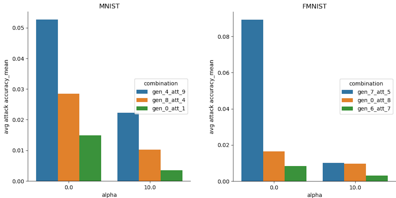
Figure 8 Results of executing the CRPA with differential privacy for the MNIST (left) and FMNIST (right) datasets. The results show that the effect of the CRPA is practically negligible due to the application of DP
