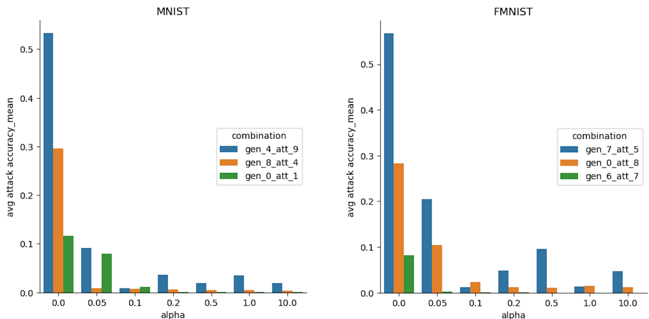
Figure 6 Results of executing the CRPA with different data distributions generated using the Dirichlet distribution for the MNIST (left) and FMNIST (right) datasets
