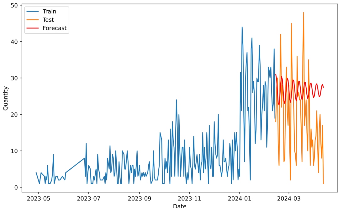
Figure 3 ARIMA forecasted material stock quantity
