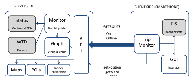
Figure 1 General architecture of the indoor navigation system
