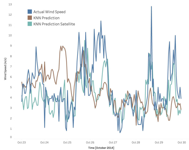
Figure 4 Comparison of actual and machine learning imputed wind speed with and without satellite information
