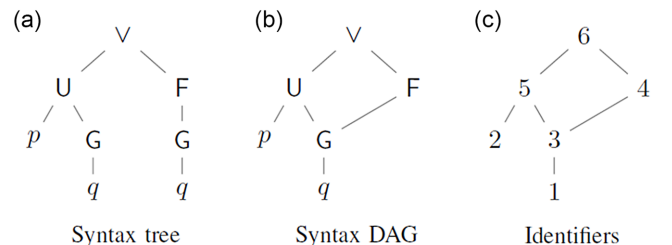
Figure 3 Syntax tree, syntax DAG, and identifiers of the syntax DAG for the LTL formula ( p \mathcal{U} \Box q \vee (\Box q) )
