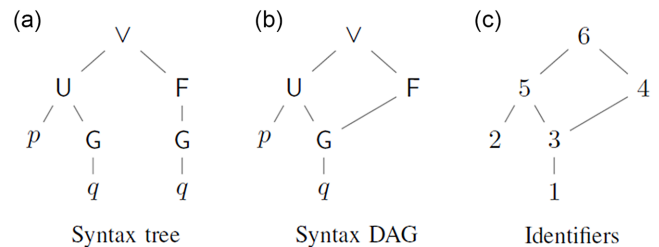
Syntax tree, syntax DAG, and identifiers of the syntax DAG for the LTL formula ( p \mathcal{U} \square q ) \vee ( \diamond(\square q) )
