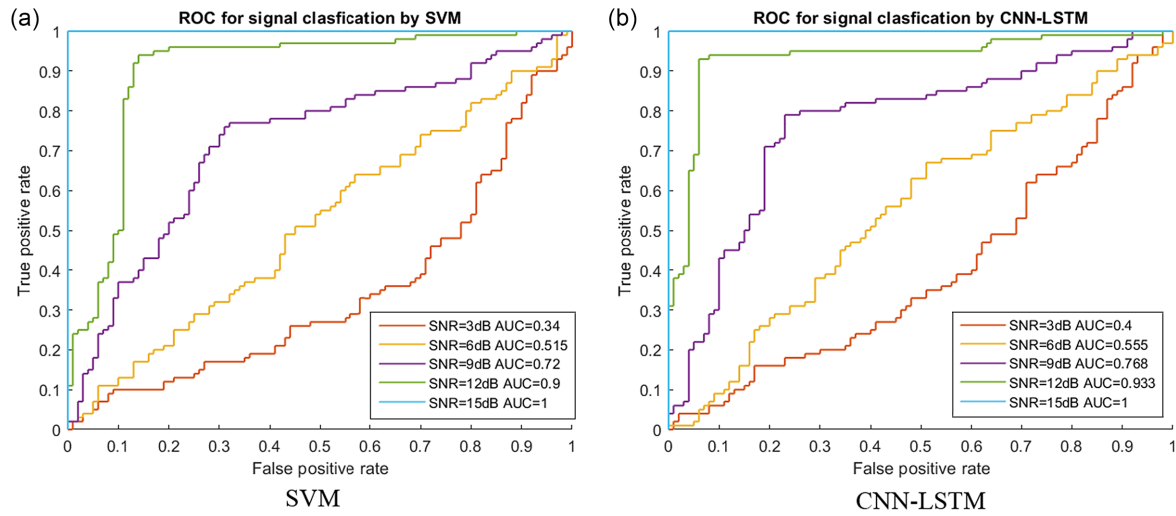
Figure 12 ROC curve for SVM and CNN-LSTM models on different noise levels
