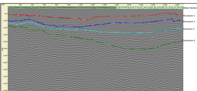
Figure 5 Seismic section with structures
