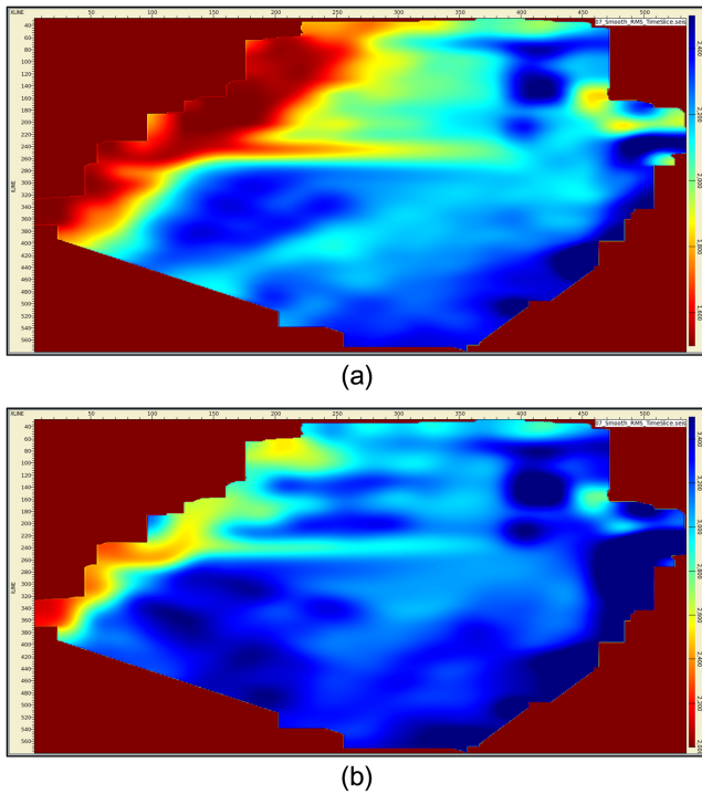
Figure 8 (a) Predicted 3D velocity volume at time 500 ms and (b) predicted 3D velocity volume at time 2000 ms
