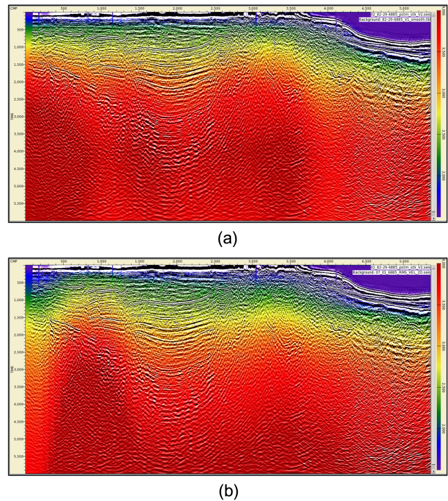
Figure 9 (a) Original picked 2D velocity overlaid on seismic and (b) predicted velocity overlaid on seismic
