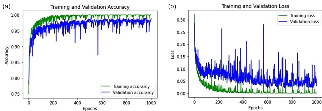
Figure 3 Training performance and validation performance
