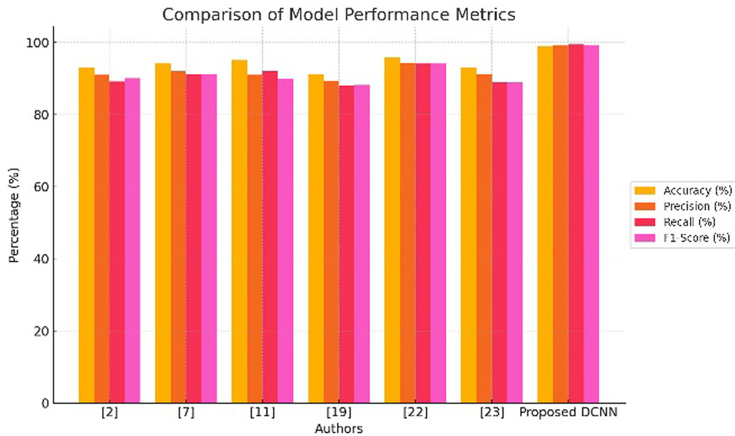
Figure 5 Comparison of proposed DCNN performance with existing techniques
