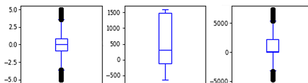
Figure 7 Box plot of each PPT variables
