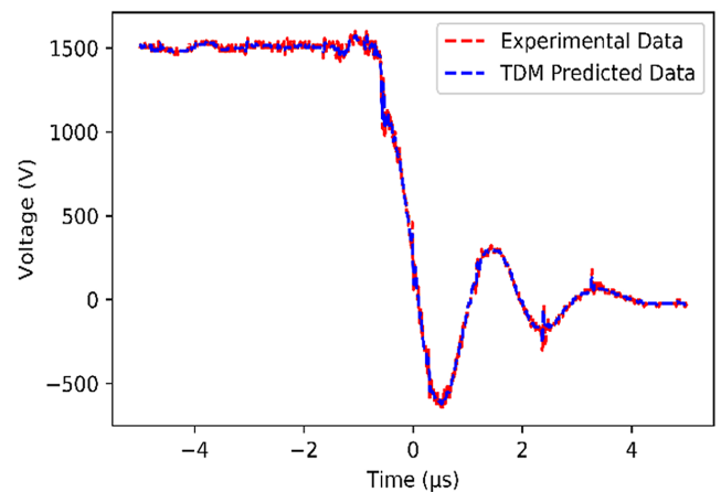
Figure 12 Experimental vs predicted voltage
