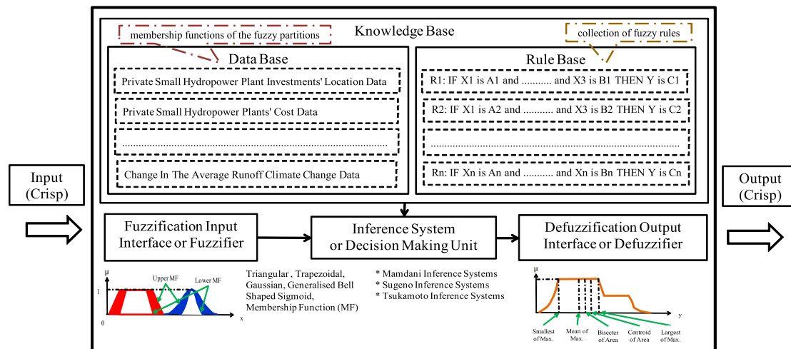
Figure 3 The current experimental one-node type-2 Mamdani's type FIS/FRBS structure
