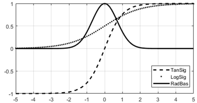
Figure 4 Activation functions
