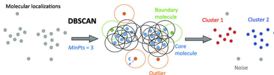
Figure 11 DBSCAN clustering
