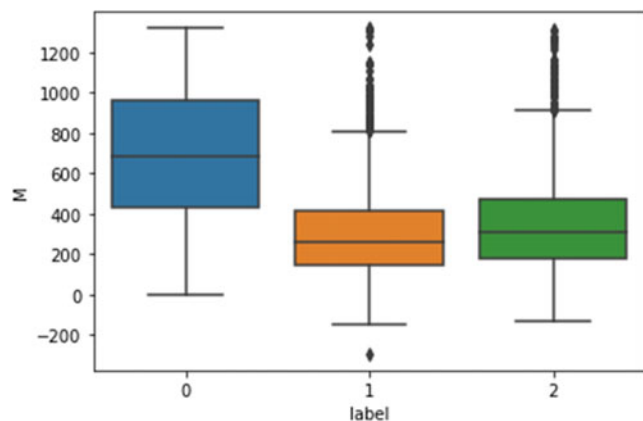
Boxplot within clusters of customers among monetary values
