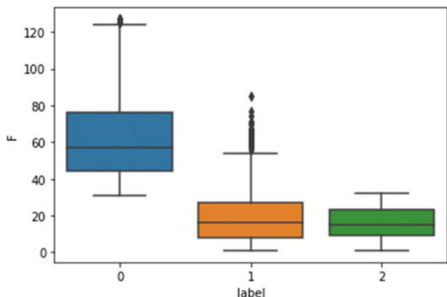
Boxplot within clusters of customers among frequency values
