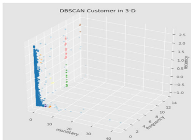
3-D clustering using DBSCAN
