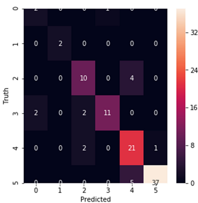
Confusion matrix for model testing using three features
