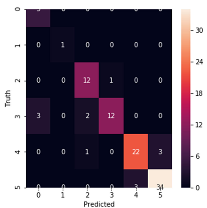
Confusion matrix for model testing using ten features
