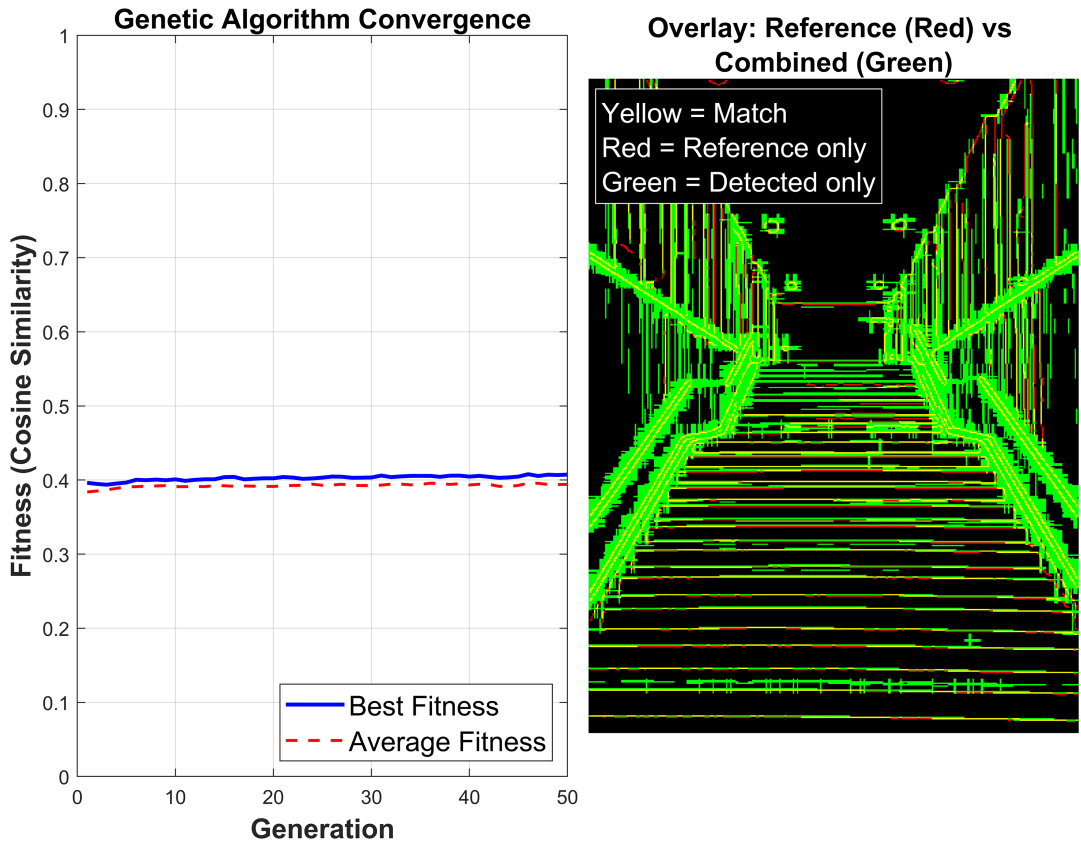
Figure 8 The dynamics of convergence of the genetic algorithm (left) and the result of comparing the contours of the stairs in the images (right): the reference one (red) and the one obtained by the combined submatrix method (green)
