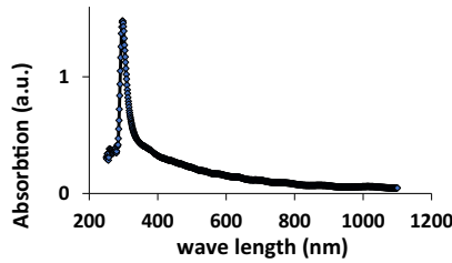
Figure 4 UV-Vis absorption spectrum of ZnO nanostructured thin film
