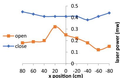
Figure 8 Open- and closed-aperture Z-scan curves of ZnO nanostructured thin film
