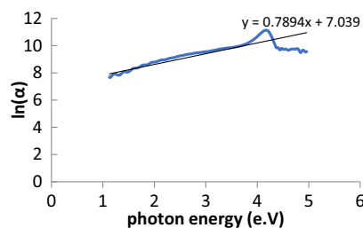
Figure 7 \ln(\alpha) versus photon energy ( h\nu ) plot for estimating Urbach energy ( E_u ) of ZnO/PS nanostructures
