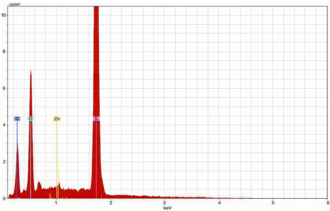
Figure 3 EDX spectrum of ZnO on PS
