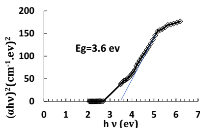
Figure 5 Tauc plot used to determine the optical band gap energy ( \sim 3.6 eV)
