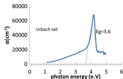
Figure 6 Absorption coefficient ( \alpha ) versus photon energy ( h\nu )
