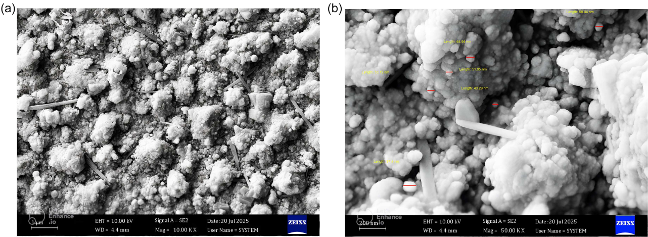
Figure 2 (a) Low-magnification and (b) high-magnification SEM images of ZnO nanostructures grown on PS
