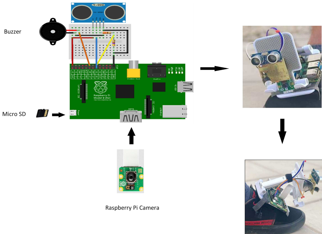
Figure 3 Overall system implementation
