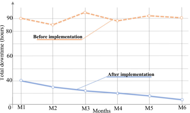
Figure 10 Monthly trend of total downtime (in hours) before and after robotic system implementation
