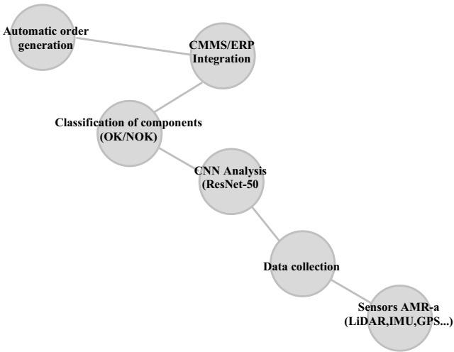
Figure 8 Workflow diagram of the integrated AMR–cobot inspection process
