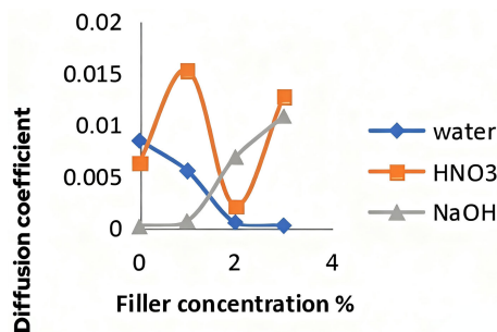
Figure 8 Diffusion coefficients as a function of filler content of all samples
