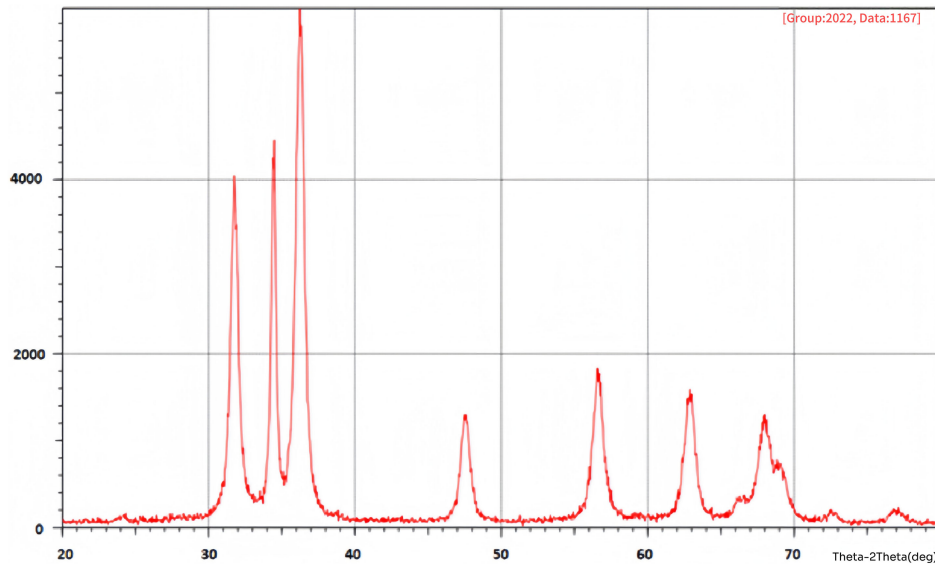
Figure 1 Typical XRD pattern of ZnONPs
