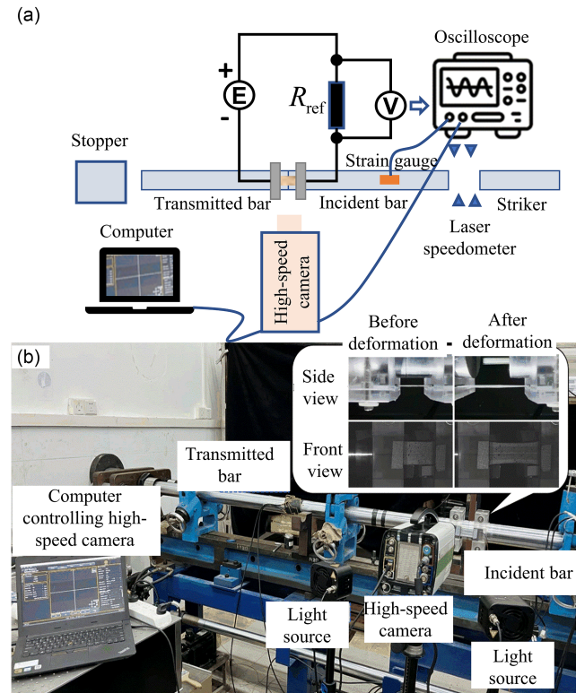
Figure 2 Dynamic loading subsystem: (a) the schematic diagram of the dynamic loading subsystem and (b) picture of the subsystem with illustrations
