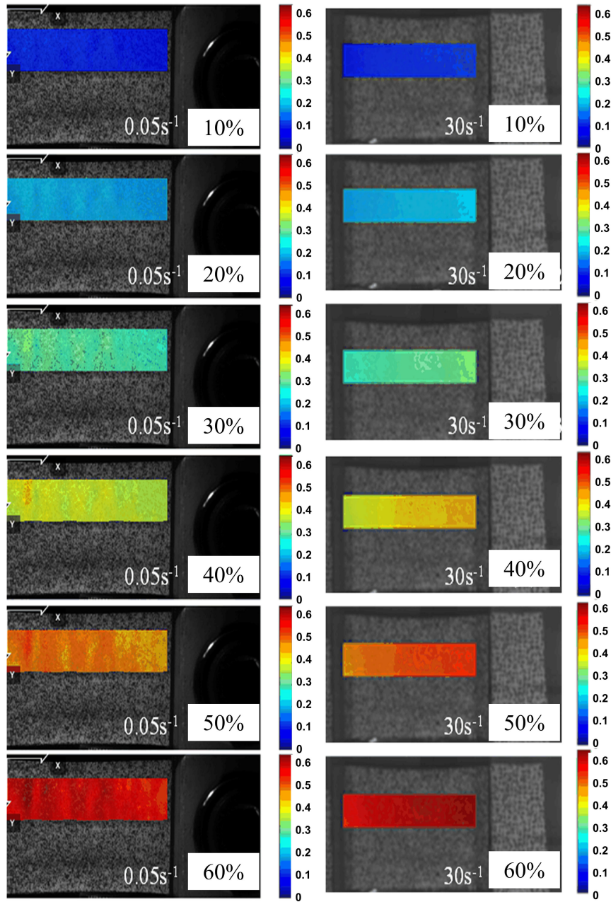
Figure 14 Contour map of sensor deformation field during tensile tests at different strains and strain rates
