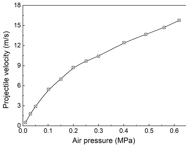
Figure 5 The relationship between the projectile velocity and the air pressure
