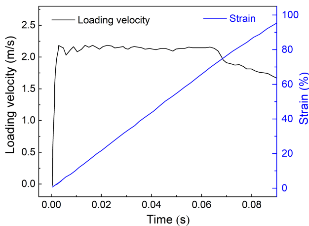
Loading velocity versus strain during dynamic loading
