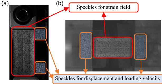
Figure 9 Typical images from high-speed camera for DIC displacement measurement: (a) quasi-static measurement, and (b) dynamic measurement
