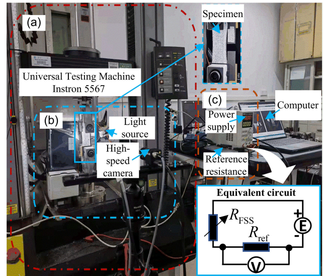
Figure 1 The quasi-static loading subsystem comprises three main components: (a) the loading unit, (b) the mechanical measurement unit, and (c) the electrical measurement unit
