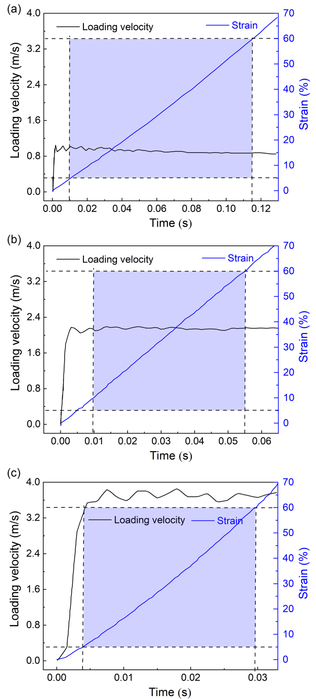
Figure 6 Time-loading velocity and time-strain curves during loadings at (a) 1.0 m/s, (b) 2.1 m/s, and (c) 3.7 m/s
