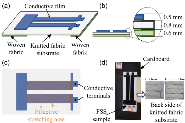
Figure 7 The configuration of FSS: (a) schematic of FSS from an oblique view, (b) schematic of sensor from a front view, (c) definition of stretching and non-stretching area, and (d) a picture of the FSS on cardboard support in black color
