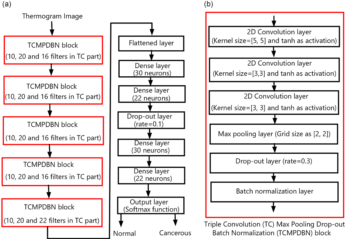
Figure 2 Architecture of the suggested DPCNN for detecting BC using thermal images
