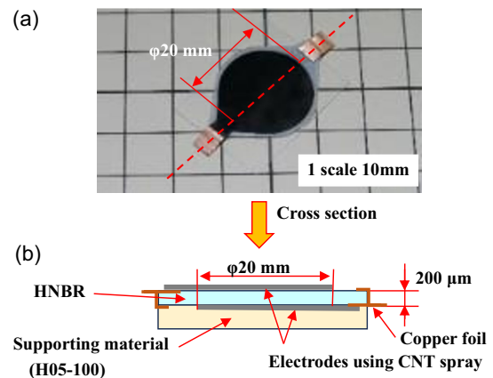
Figure 7. The prototype of a DEPS using the improved HNBR: (a) photograph of the DEPS, and (b) a cross-section of the DEPS
