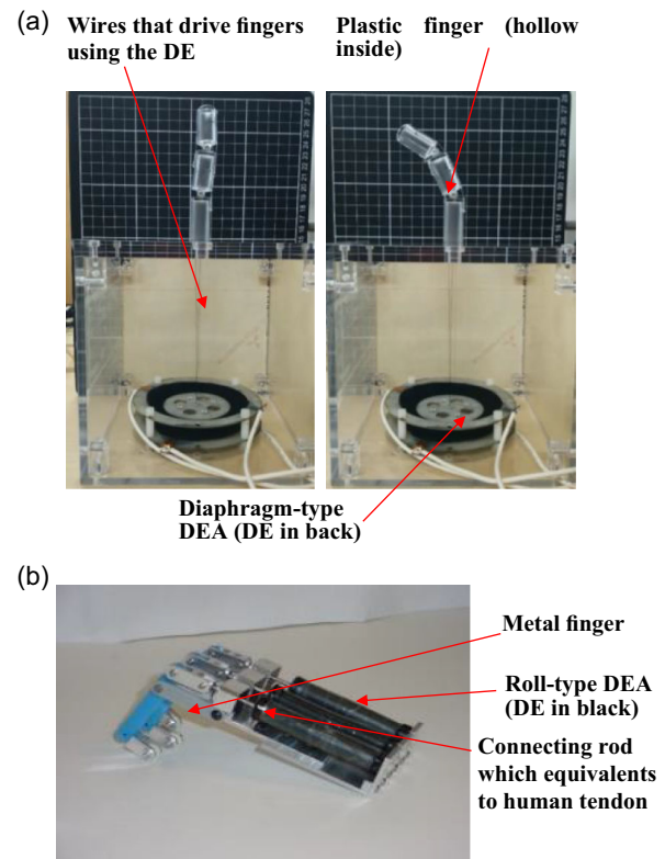
Figure 2. Small robot hands
