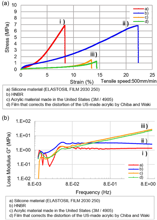
Figure 14. (a) SS curves and (b) viscoelastic properties of the four films: materials used: (i) silicone ELASTSIL film/2030-250, (ii) HNBR, and (iii) acrylic 3M4905, and strain-relieved film of 3M4905
