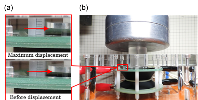
Figure 1. Diaphragm-type DE actuator capable of lifting an 8 kg weight (black part: diameter 8 cm): (a) DE actuator before (bottom) and after (top) actuation, and (b) DE actuator actuated and stretched vertically
