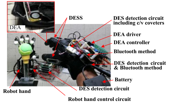
Figure 10. DE motion feedback system: the small diaphragm DE actuator on the top is a device that operates when the robot's finger touches a target part, creating a sense of touch
