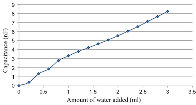
Figure 4. Moisture sensor
