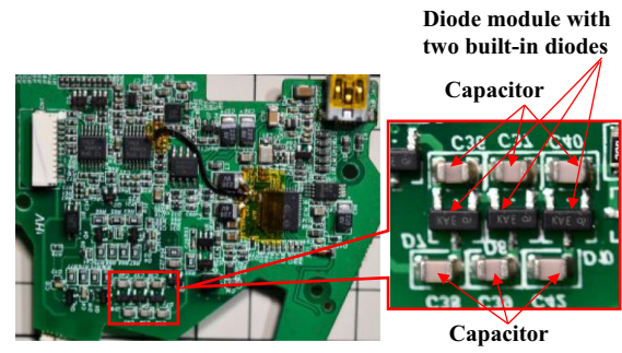
Figure 6. Circuit board for headphones with a DE vibrator
