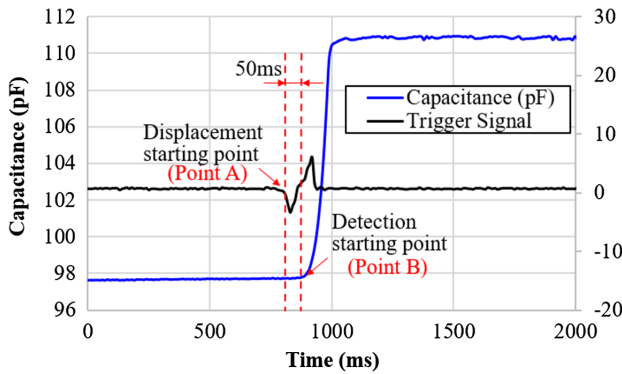
Figure 9. Changes in measured capacitance
