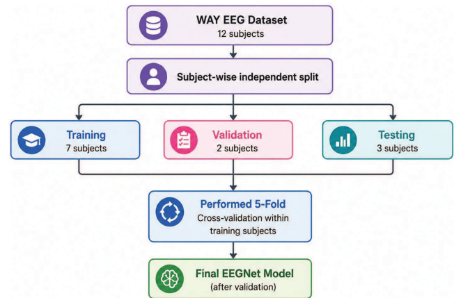
Figure 2 Partitioning of the WAY EEG dataset into training, validation, and test subjects
