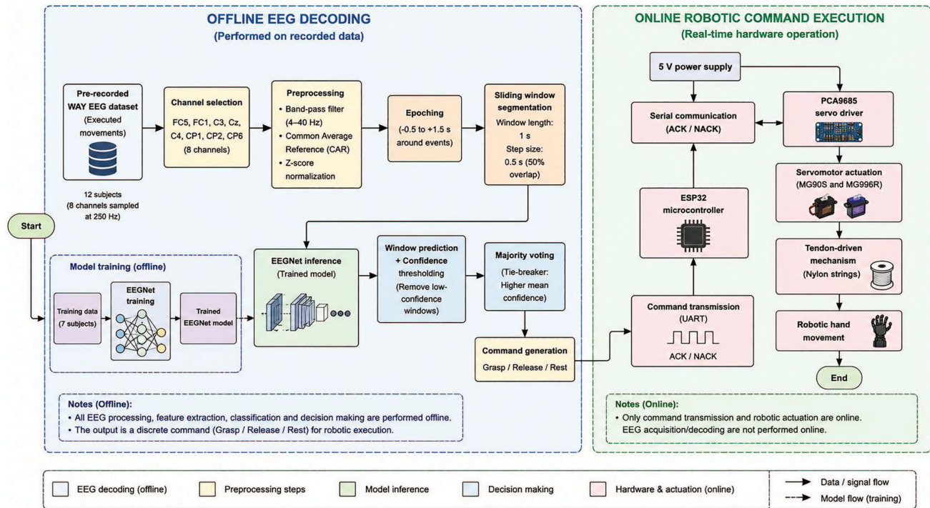
Figure 1 System architecture workflow for tendon-driven robotic hand actuation through BCI
