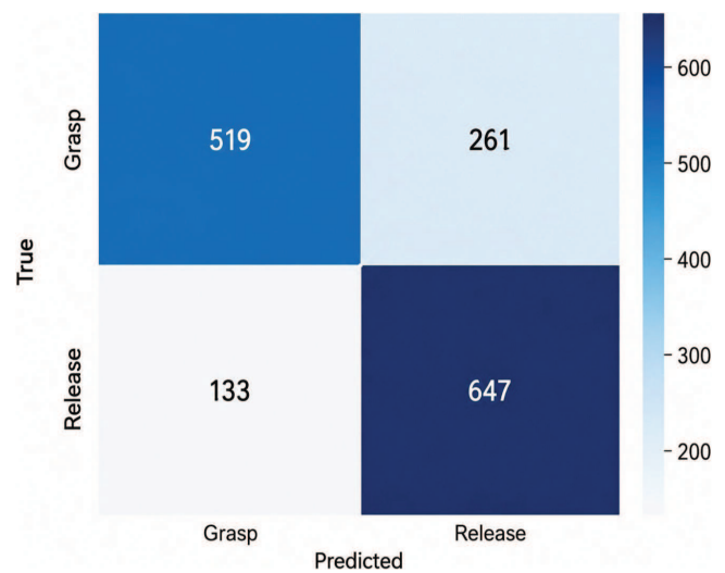
Figure 7 Confusion matrix for EEGNet grasp/release classification
