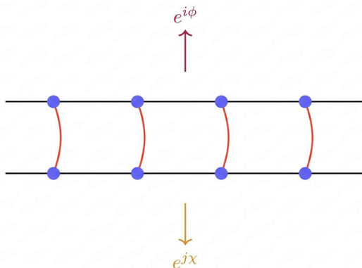
Figure 2. Biphoton entanglement between parallel axons, modulated by the spiral-time sectors \phi (emotional phase) and \chi (identity depth). This links the biological experiments to the HLV operator
