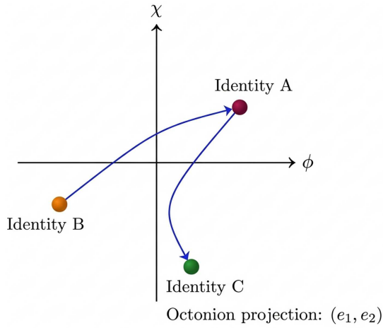
Figure 3. Octonionic projection of the identity field on the (\phi, \chi) plane. Attractors correspond to DLHR A4/A5 states, and transitions arise from non-associative interaction terms
