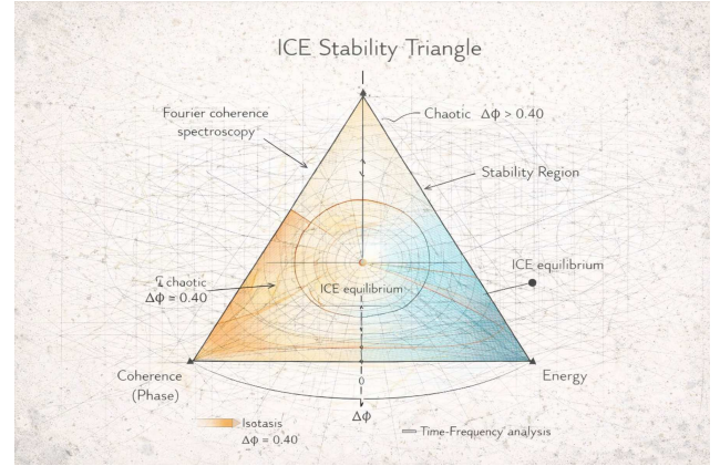
Figure 5. ICE stability triangle illustrating the information–coherence–energy (ICE) balance. The central region corresponds to isostatic stability, while phase instability emerges beyond the critical threshold \Delta\Phi \approx 0.40
