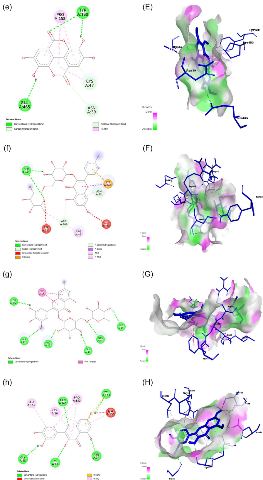
Figure 5. On the left, two-dimensional diagrams of the binding interactions of (a) L8, (b) L18, (c) L21, (d) L24, (e) L25, (f) L26, (g) L29, and (h) L32 with the active site residues of the COX-2 enzyme are shown. Magenta circles indicate polar amino acids, green circles indicate nonpolar amino acids, orange circles indicate positively charged amino acids, red circles represent negatively charged amino acids, and yellow circles denote aromatic residues. On the right, three-dimensional binding poses with hydrogen bonding of (A) L8, (B) L18, (C) L21, (D) L24, (E) L25, (F) L26, (G) L29, and (H) L32 with the active site residues of the COX-2 protein are shown. Ligand atoms are depicted with ball-and-stick models (blue color), and protein residues are represented with stick models.
