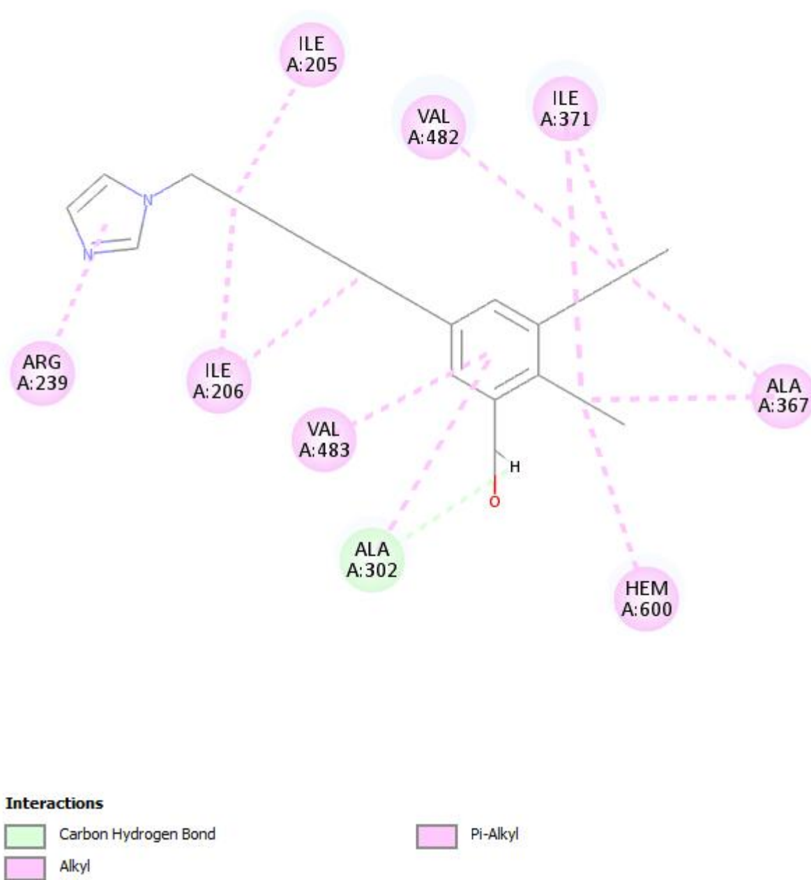
Supplementary Figure 15. 2D interactions of compound 305 within active pocket of 3ruk
