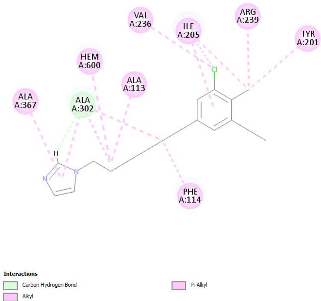
Supplementary Figure 1. 2D interactions of compound 52 within active pocket of 3ruk
