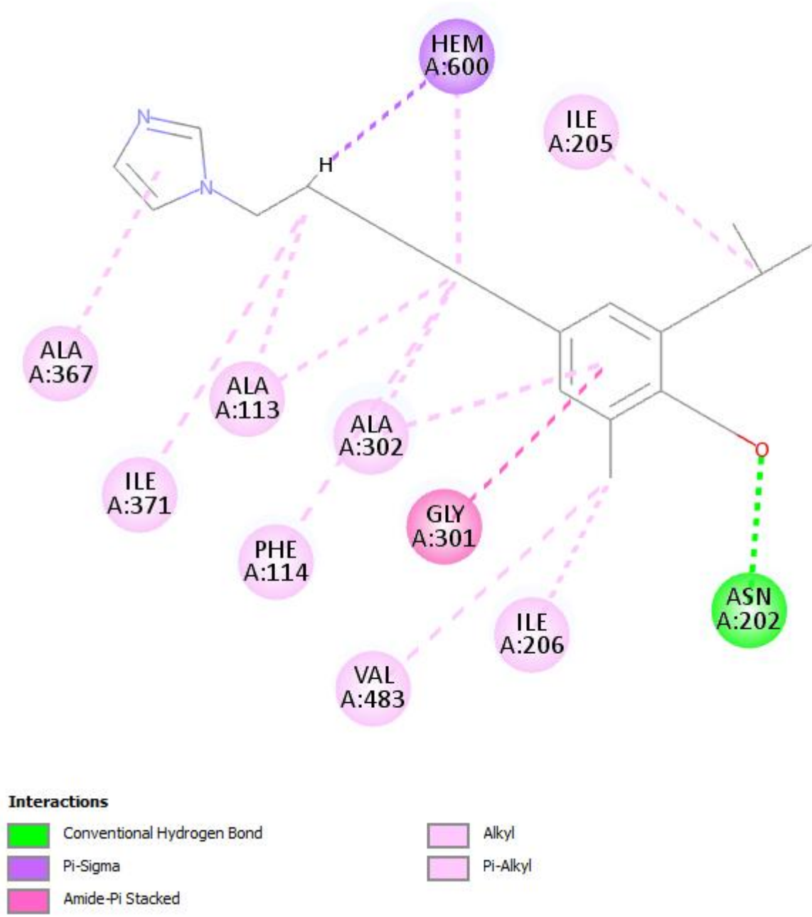
Supplementary Figure 22. 2D interactions of compound 441 within active pocket of 3ruk
