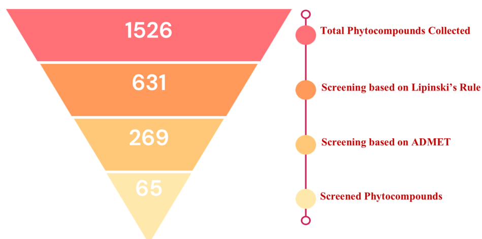
Figure 2. Screening process of phytocompounds
