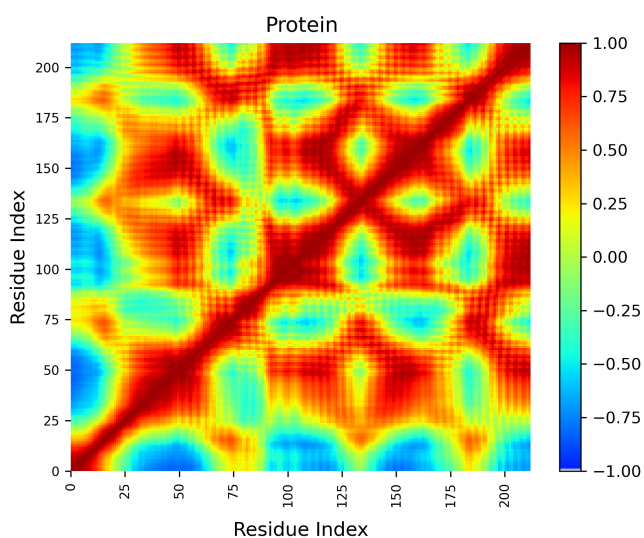
Figure 7. Heat map of NF-kappa105_6-prenylaringenin complex
