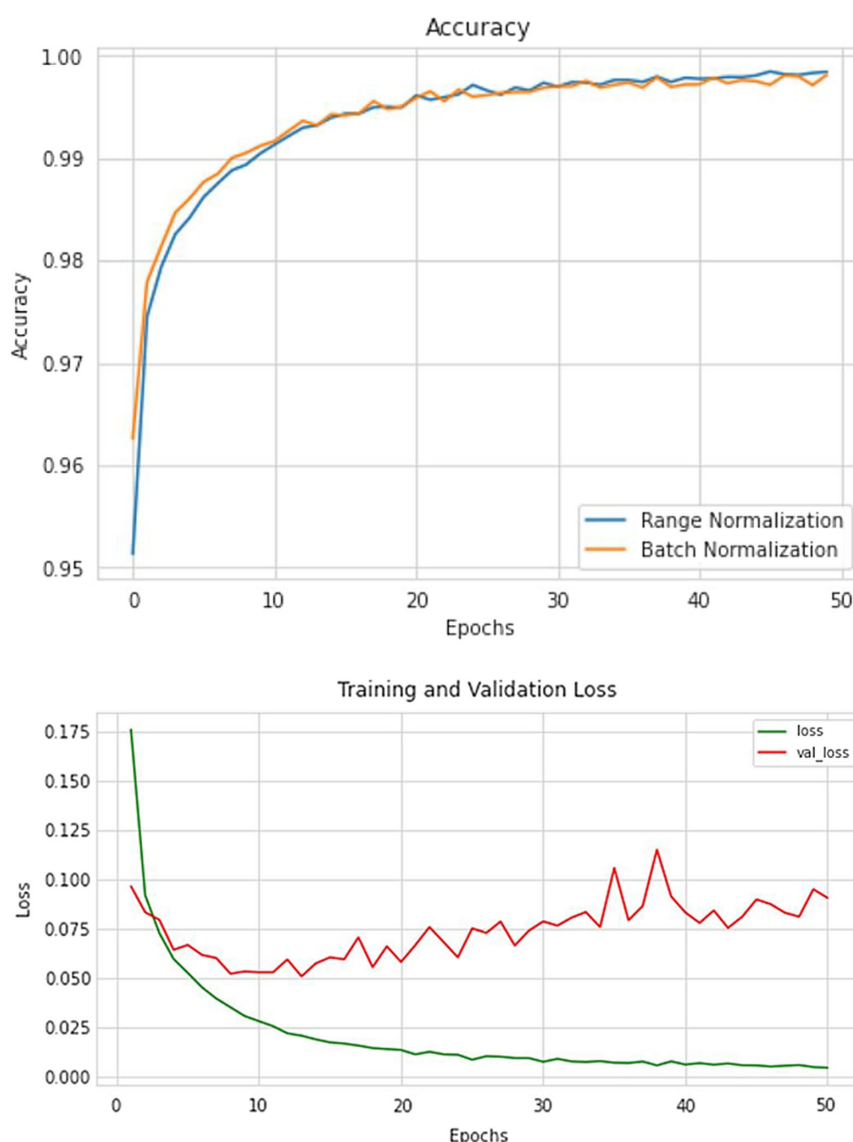
Figure 4. Classification accuracy and cross-entropy loss of batch normalization versus range normalization
