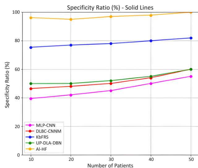
Figure 5. Specificity ratio (%)
