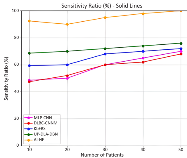
Figure 4. Sensitivity ratio (%)
