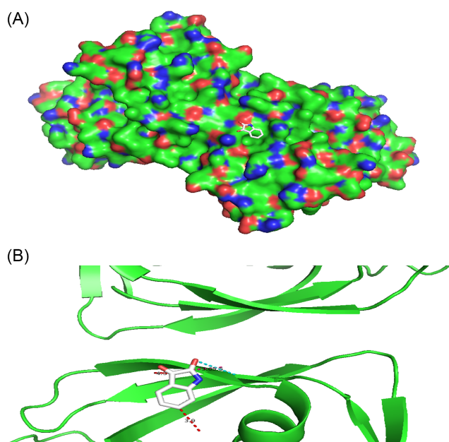
Figure 4. Peptide deformylase-1-[(4-fluorophenyl) methyl] indole-2,3-dione interaction. (A) Surface representation of peptide deformylase-1-[(4-fluorophenyl) methyl] indole-2,3-dione interaction (Figure courtesy of the authors). (B) 3D representation of peptide deformylase-1-[(4-fluorophenyl) methyl] indole-2,3-dione interaction. (Figure courtesy of the authors)
