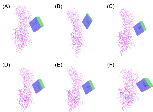
Figure 3. Grid boxes of ligands (figures courtesy of the authors). (A) 1-[(4-fluorophenyl) methyl] indole-2,3-dione. (B) 5-chloro-1-(2-phenylethyl) indole-2,3-dione. (C) 7-bromo-1-(thiophen-3-ylmethyl) indole-2,3-dione. (D) 1-[(5-bromothiophen-2-yl) methyl] indole-2,3-dione. (E) 7-bromo-1-(thiophen-2-ylmethyl) indole-2,3-dione. (F) 5-ethylthieno[2,3-f] indole-6,7-dione
