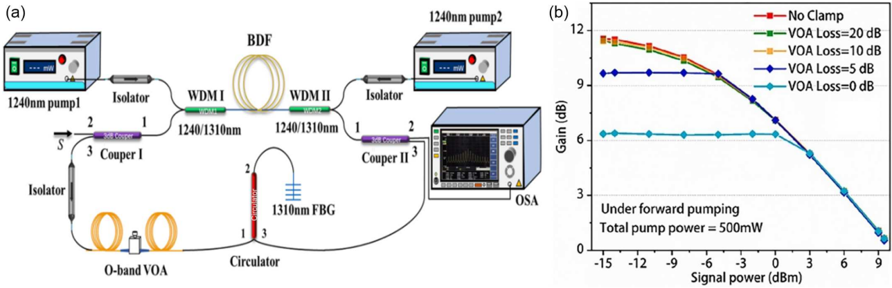
Figure 14 The (a) scheme and (b-c) gain-clamped operation of BDFA with adjustable semi-ring semi-linear cavity
