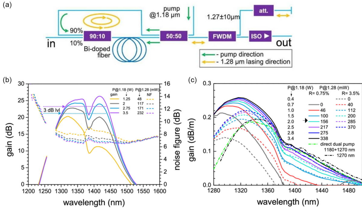
Figure 14 The (a) scheme and (b-c) gain-clamped operation of BDFA with adjustable semi-ring semi-linear cavity
