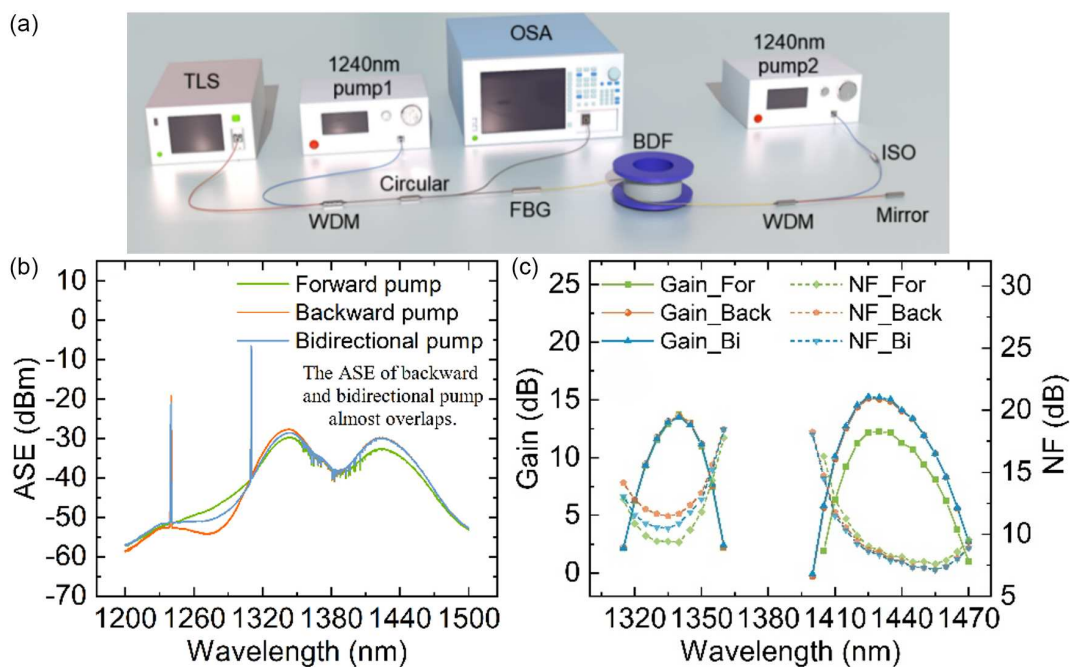
Figure 18 (a) The scheme, (b) ASE, and (c) gain spectra of bandwidth-expanding dual-pass linear cavity gain control BDFA
