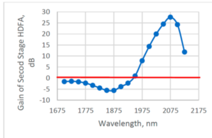
Figure 5 Gain (attenuation) of the second HDFA stage as a function of signal wavelength for 0 dBm signal input power. The 0 dB gain or transparency line is shown in red
