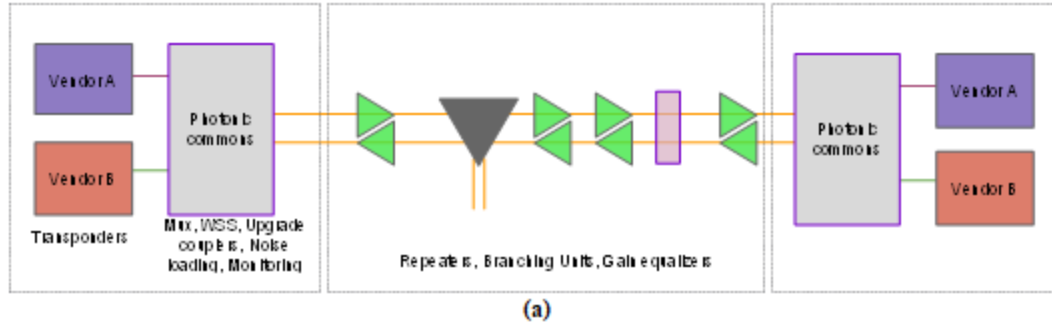
Figure 11 (a) Overall optical architecture for the future 2000 nm DWDM lightwave transmission system under study and (b) OSNR evolution in the 2000 nm DWDM lightwave system for a cascade of N identical amplified sections with amplifier gain = span loss
