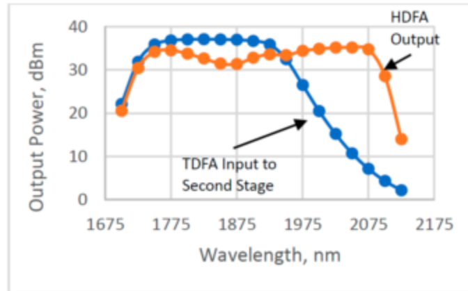
Figure 4 Output powers from the first TDFA stage (blue) and second HDFA stage (orange) as a function of signal wavelength from 1700 nm to 2125 nm
