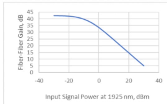
Figure 10 Device fiber-fiber gain as a function of input signal power at 1925 nm for the wideband hybrid TDFA-HDFA of Figure 1
