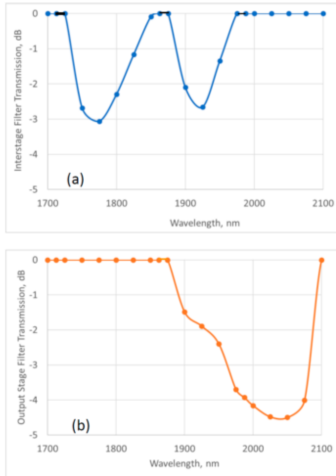
Figure 6 (a) Spectral characteristics of interstage gain flattening filter inserted after the first Tm-doped stage and (b) output gain flattening filter inserted after the second Ho-doped stage
