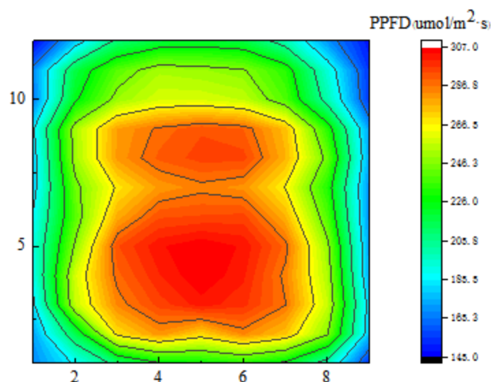
Figure 3 Light intensity distribution in lettuce planting plane
