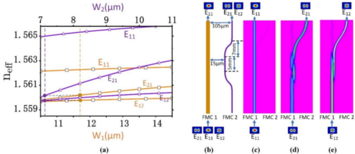
Figure 3 (a) The effective refractive indices of different TE-polarized guide modes change with the core width of FMC 1 (orange color) and the core width of FMC 2 (purple color) at 1550 nm, where the chosen widths for FMC 1 and FMC 2 are fixed at w_1=11.7\ \mu\text{m} and w_2=7.2\ \mu\text{m} for phase-matched that is highlighted by thin vertical lines. (b) The top view of the waveguide structure built in Rsoft CAD and the propagation paths with (c) the E_{11} , (d) the E_{21} , and (e) the E_{12} modes launched into FMC 1
