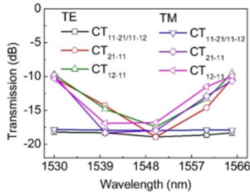
Figure 12 Crosstalks of the mode-group (de)multiplexer caused by the E_{11} mode and the residual power of the E_{21} and E_{12} modes
