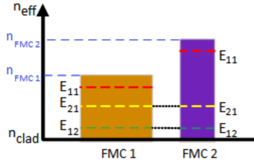
Figure 2 The phase-matching condition for the E_{21} mode and E_{12} mode between FMC 1 and FMC 2, where the effective refractive index of the E_{21} and E_{12} modes in FMC 1 is phase-matched that in FMC 2
