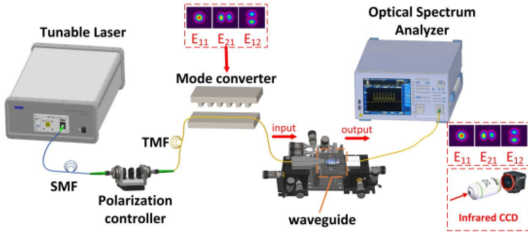
Figure 9 Experimental setups for the device measurement
