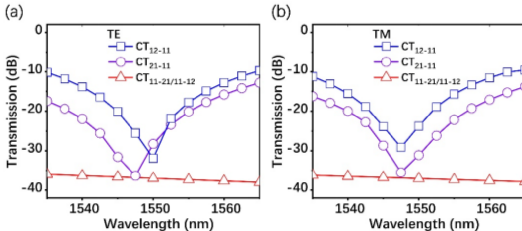
Figure 5 The crosstalk of the residual power with launching the E_{21} , and E_{12} modes into the FMC 1 and the weak coupling of the E_{11} mode from FMC 1 to FMC 2 for (a) the TE, (b) the TM polarizations
