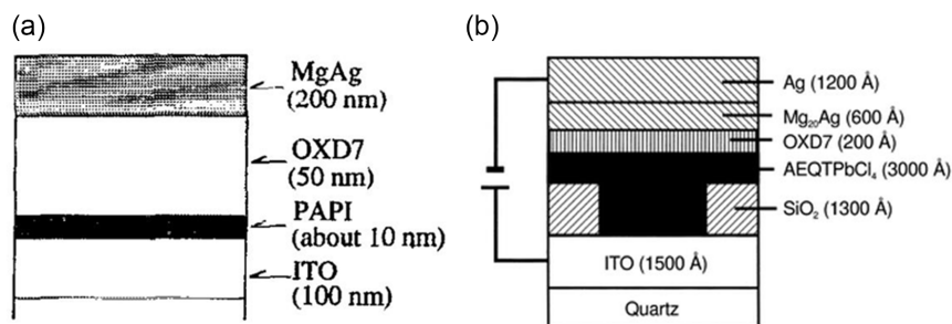
Figure 2 Self-assembled low-dimensional MHP MQWs before the Renaissance. (a) Low-temperature operating LED with phenethylammonium lead iodide (noted as PAPI ( C_6H_5C_2H_4NH_3 ) _2PbI_4 ) and (b) room temperature operating LED with AEQTPbCl _4 ( H_3NC_2H_4C_{16}H_8S_4C_2H_4NH_3PbCl_4 )
