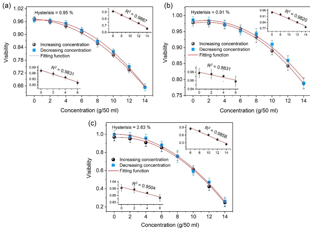
Repeatability and hysteresis analysis of the proposed interferometric polarimeter for one full cycle of the increasing and decreasing concentrations for (a) sucrose, (b) glucose, and (c) fructose. Each parabolic curve can be divided into two linear regions: 0 – 6 g/50 ml and 6 – 14 g/50 ml, as shown in the inset of the plots
