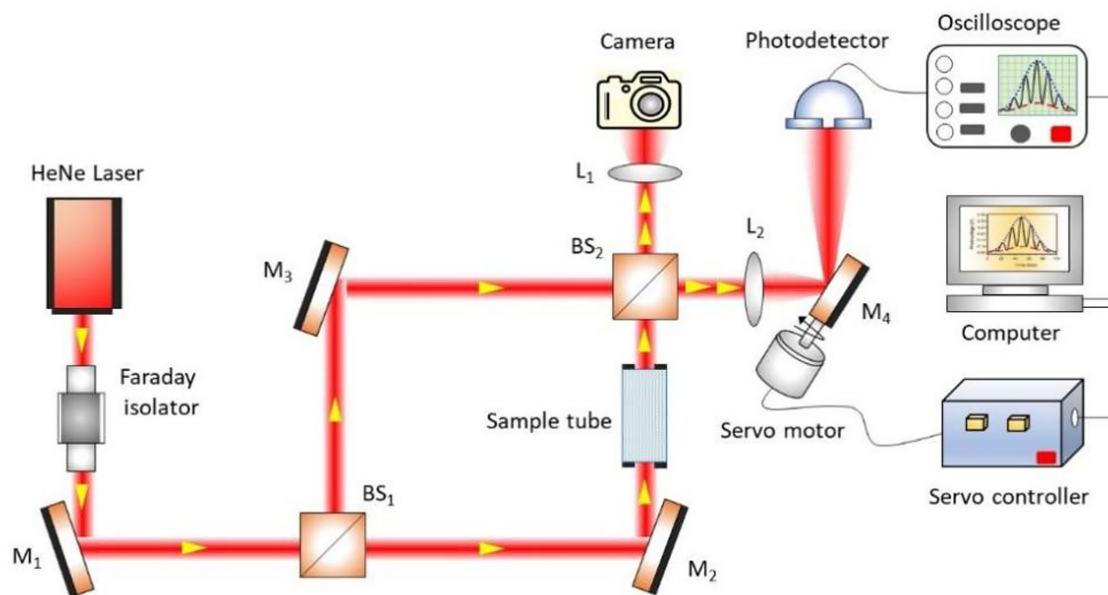
Figure 1 Schematic diagram of the experimental setup for interference fringes scan interferometric polarimeter. The labels M_1 , M_2 , M_3 , and M_4 represent aluminum-coated reflecting mirrors, BS_1 and BS_2 are the non-polarizing (50:50) beam splitters, and L_1 and L_2 are the convex lenses
