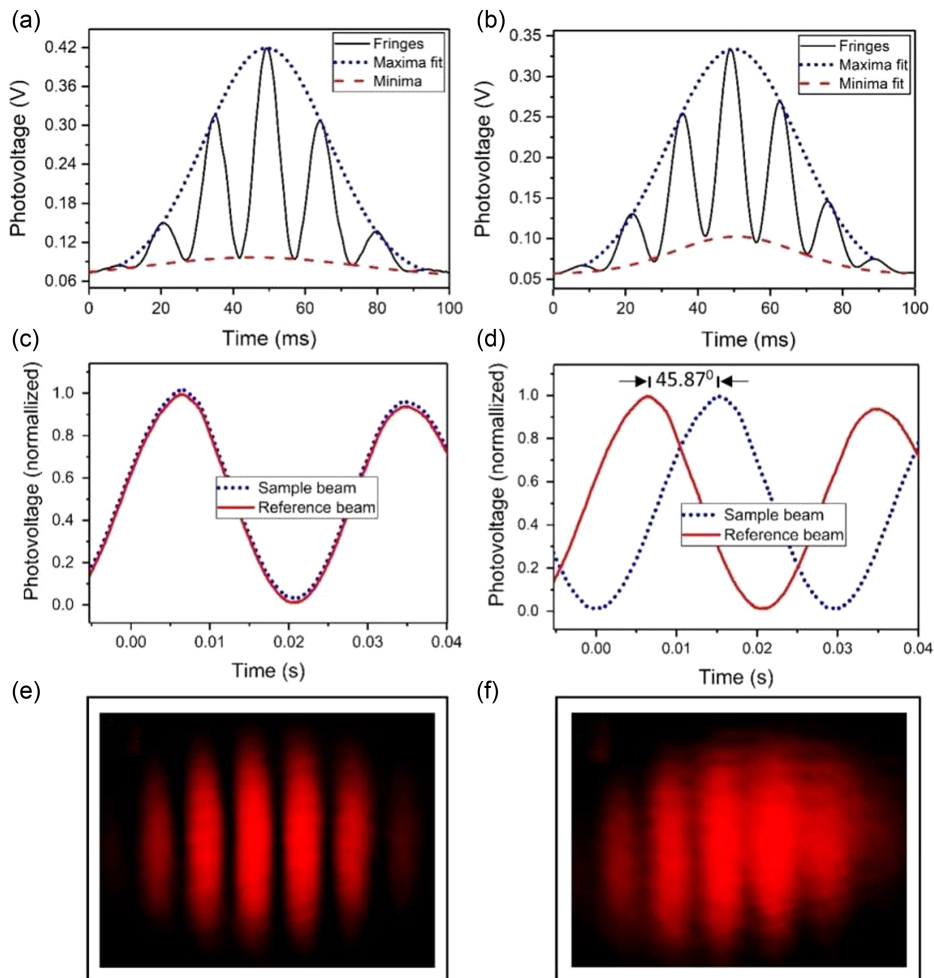
Figure 3 Intensity profile of interference patterns recorded for (a) DI water (b) 14 g/50 ml of sucrose solution. Optical rotation observed by PLRA polarimeter for (c) DI water (d) 14 g/50 ml of sucrose solution. Images of interference patterns captured by the reflex camera for (e) DI water and (f) 14 g/50 ml of sucrose solution
