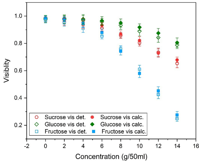
Figure 4 Variations in visibilities with change in sugar concentration as determined from maxima and adjacent minima of the interference patterns using Equation (2) and calculated based on polarimetric rotation and intensity of the transmitted beam through the sugar sample using Equation (3)
