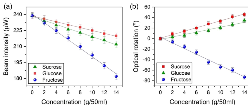
(a) Intensity variation of the sample beam after passing through the sample tube with different concentrations of sugar solutions. (b) Optical rotation in the polarization of the sample beam caused by the sugar solutions at different concentrations. Solid lines over the corresponding scatters show the linear curve fitting
