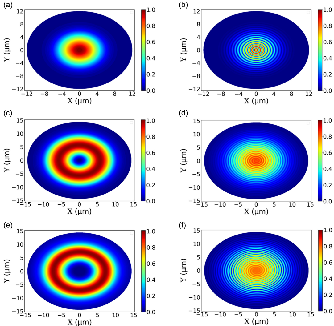
Figure 6 Intensity distribution of (a) HE_{11} , (c) HE_{21} , and (e) HE_{31} core modes. Interference pattern of OAM_{+l} for (b) HE_{11}^{\text{even}} + iHE_{11}^{\text{odd}} , (d) HE_{21}^{\text{even}} + iHE_{21}^{\text{odd}} and (f) HE_{31}^{\text{even}} + iHE_{31}^{\text{odd}}
