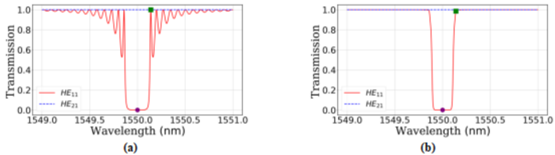
Figure 5 Transmission spectrum for HE_{11} core mode- HE_{19} cladding mode coupling (red) and HE_{21} core mode- HE_{19} cladding mode coupling (blue) (a) without apodization and (b) with pure cosine apodization. Intensity of (HE_{21} + HE_{11}) at the (c) resonance wavelength and (d) at edge of transmission point of bandwidth
