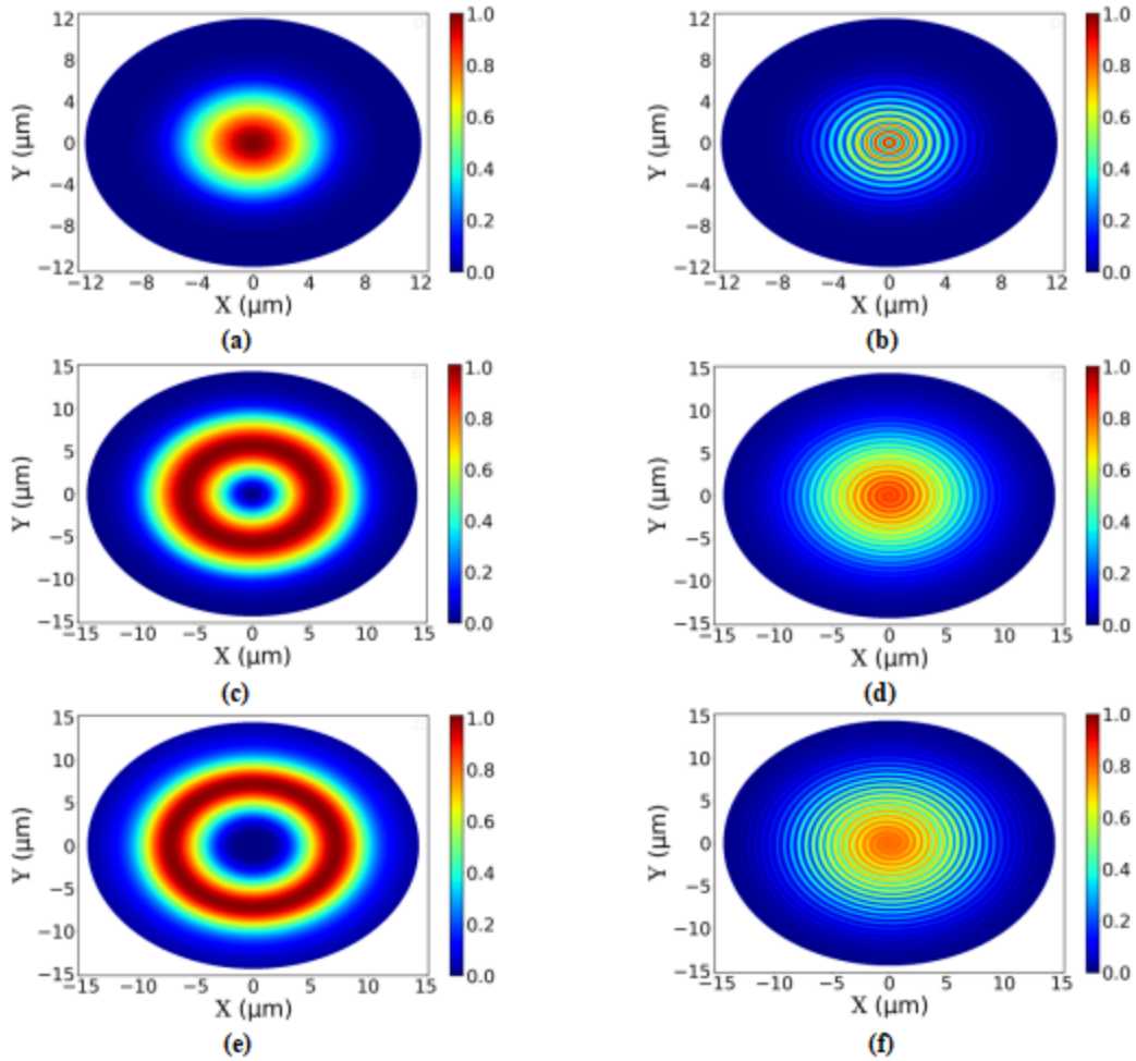
Figure 6 Intensity distribution of (a) HE_{11} , (c) HE_{21} and (e) HE_{31} core modes. Interference pattern of OAM ±1 for (b) HE_{11}^{even} + iHE_{11}^{odd} , (d) HE_{21}^{even} + iHE_{21}^{odd} and (f) HE_{31}^{even} + iHE_{31}^{odd}
