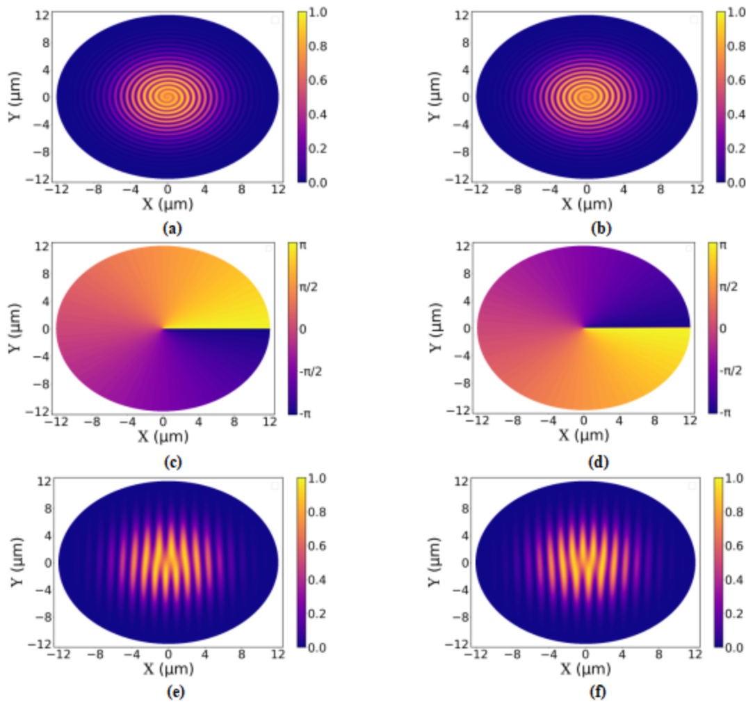
Figure 1 Coaxial interference pattern of (a) OAM_{-1} and (b) OAM_{+1} with a reference Gaussian beam. Phase pattern of generated (c) OAM_{-1} and (d) OAM_{+1} . Off-axial interference pattern of (e) OAM_{-1} and (f) OAM_{+1} with Gaussian beam
