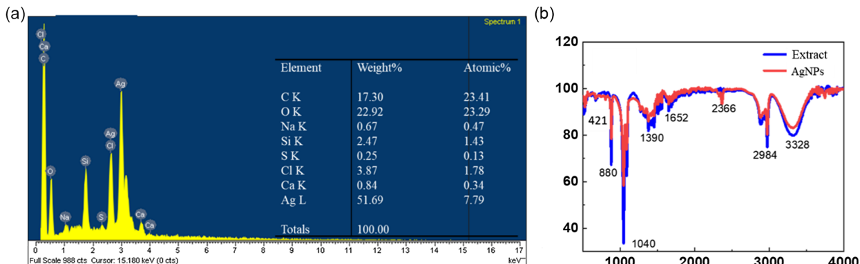
(a) EDS analysis of AgNPs and (b) FT-IR spectra of AgNPs synthesized using Pterospermum Diversifolium semi-solid extract
