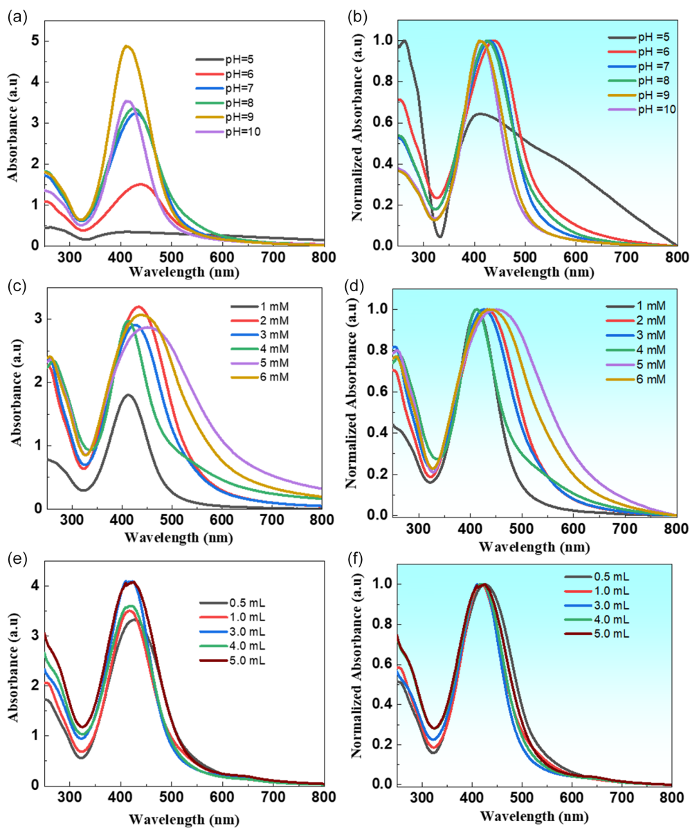
Figure 1 (a–b) Absorption spectra and normalized absorption spectra of AgNP solutions when pH changes and (c–d) AgNO 3 concentration changes, and (e–f) extract volume changes
