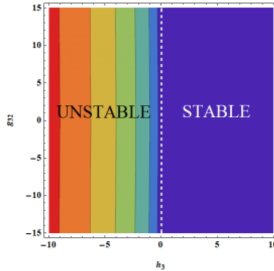
Figure 1 Modulationally stable and unstable zones in the g_{32} - h_3 Plane with other nonlinear parameters. The properties of MI are changed dramatically by g_{32} and h_3
