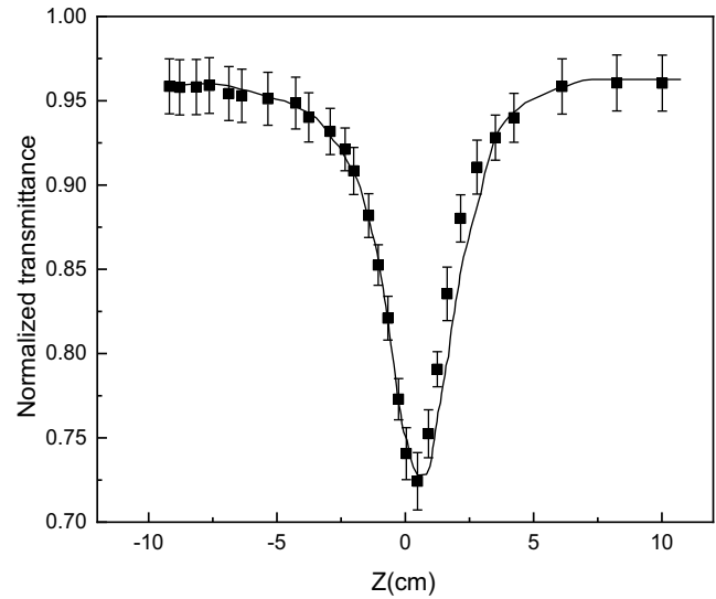
Z-scan measurement with open aperture of Cu-NPs in deionized water
