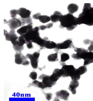
Figure 3 TEM image of Cu nanoparticle soluble in water
