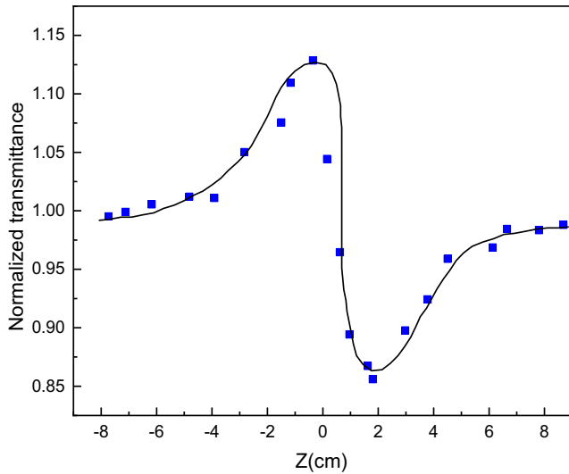
Figure 6 Z-scan measurement with closed aperture of Cu-NPs in deionized water
