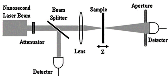
Figure 1 The Z-scan optical setup
