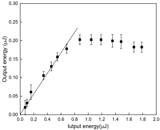
Optical limiting performance for the copper nanoparticles
