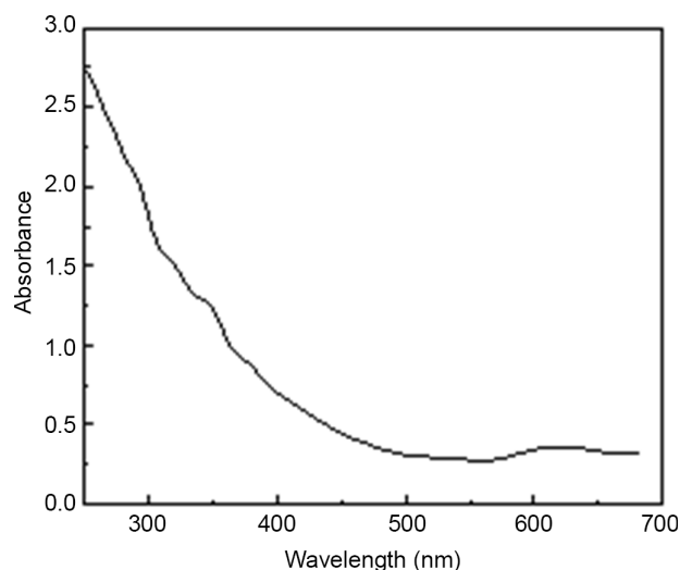
Figure 2 Absorption spectrum of the Cu nanoparticle suspension
