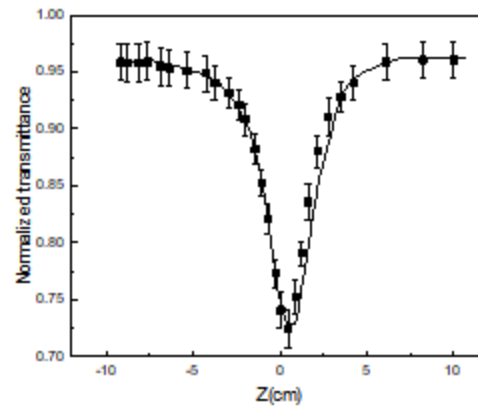
Figure 5 Z-scan measurement with open aperture of Cu-NPs in deionized water
