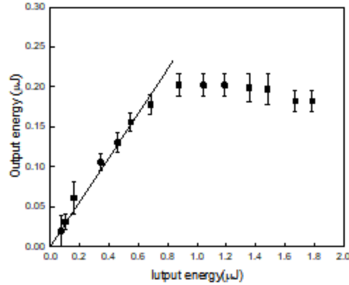
Figure 4 Optical limiting performance for the copper nanoparticles
