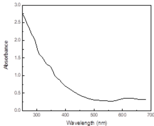
Figure 2 Absorption spectrum of the Cu nanoparticle suspension
