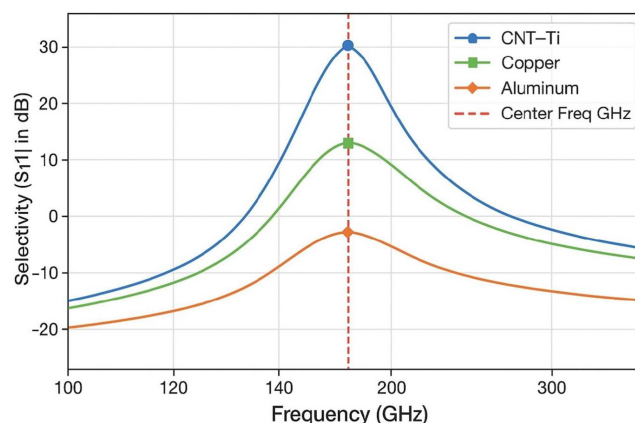
Figure 6 Efficiency comparisons of CNT-Ti and conventional patches
