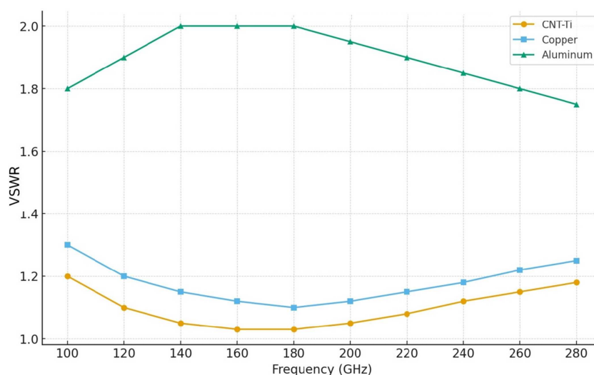
Figure 4 VSWR comparisons of CNT-Ti and conventional patches
