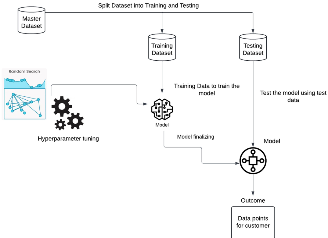
Figure 2 Hyperparameter optimization
