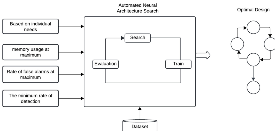
Figure 1 NAS architecture
